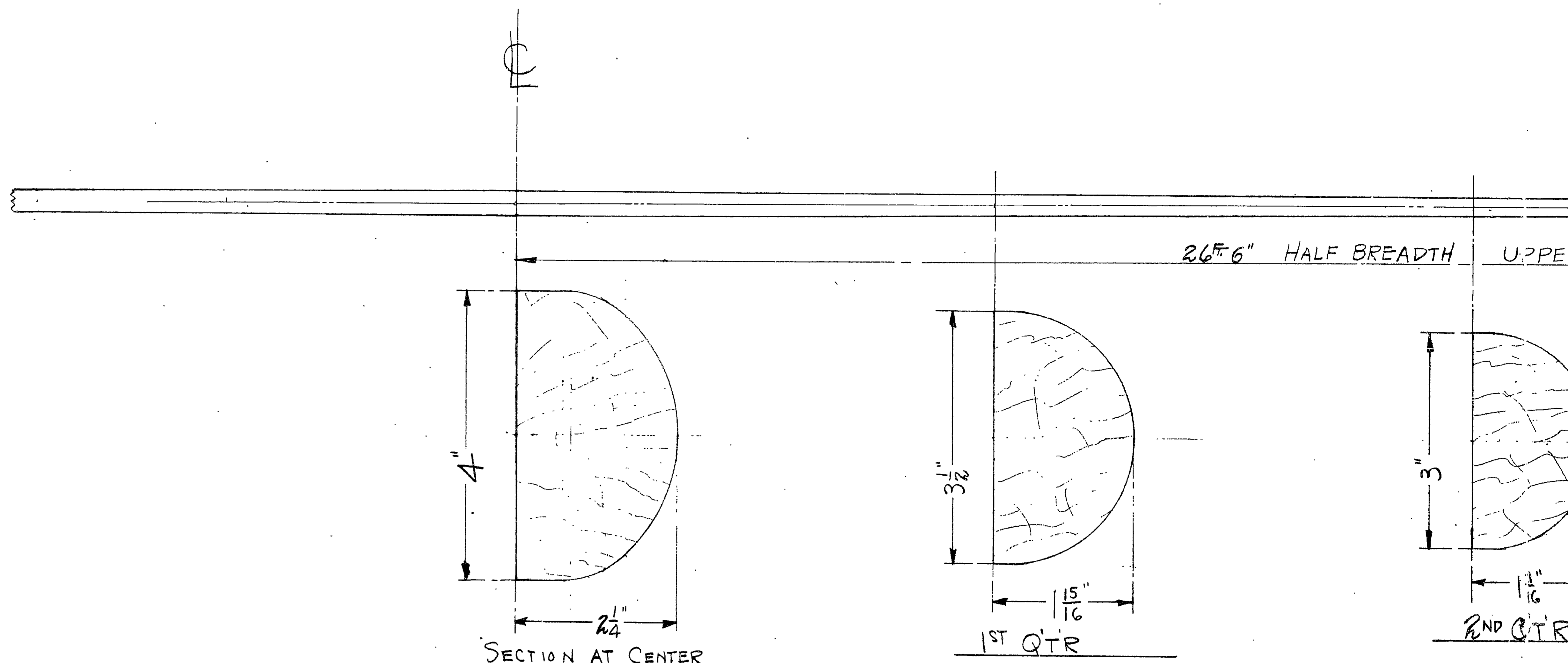
FIRST-BEADING BELOW SPAR DECK SCALE: 1" = 12" STEAMED AND BENT WHITE ONE REQ'D
