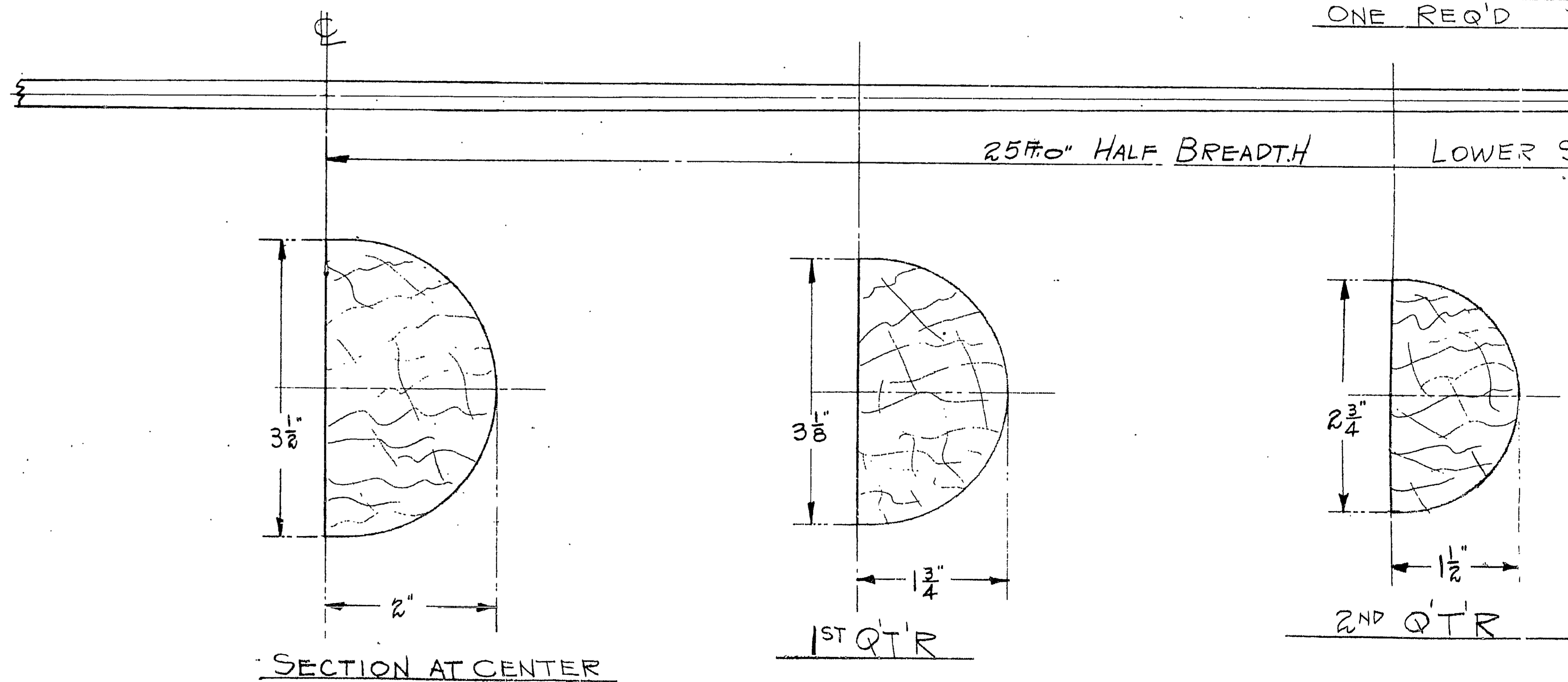
SECOND-BEADING BELOW SPAR DECK SCALE: 1" = 12" STEAMED AND BENT ONE
