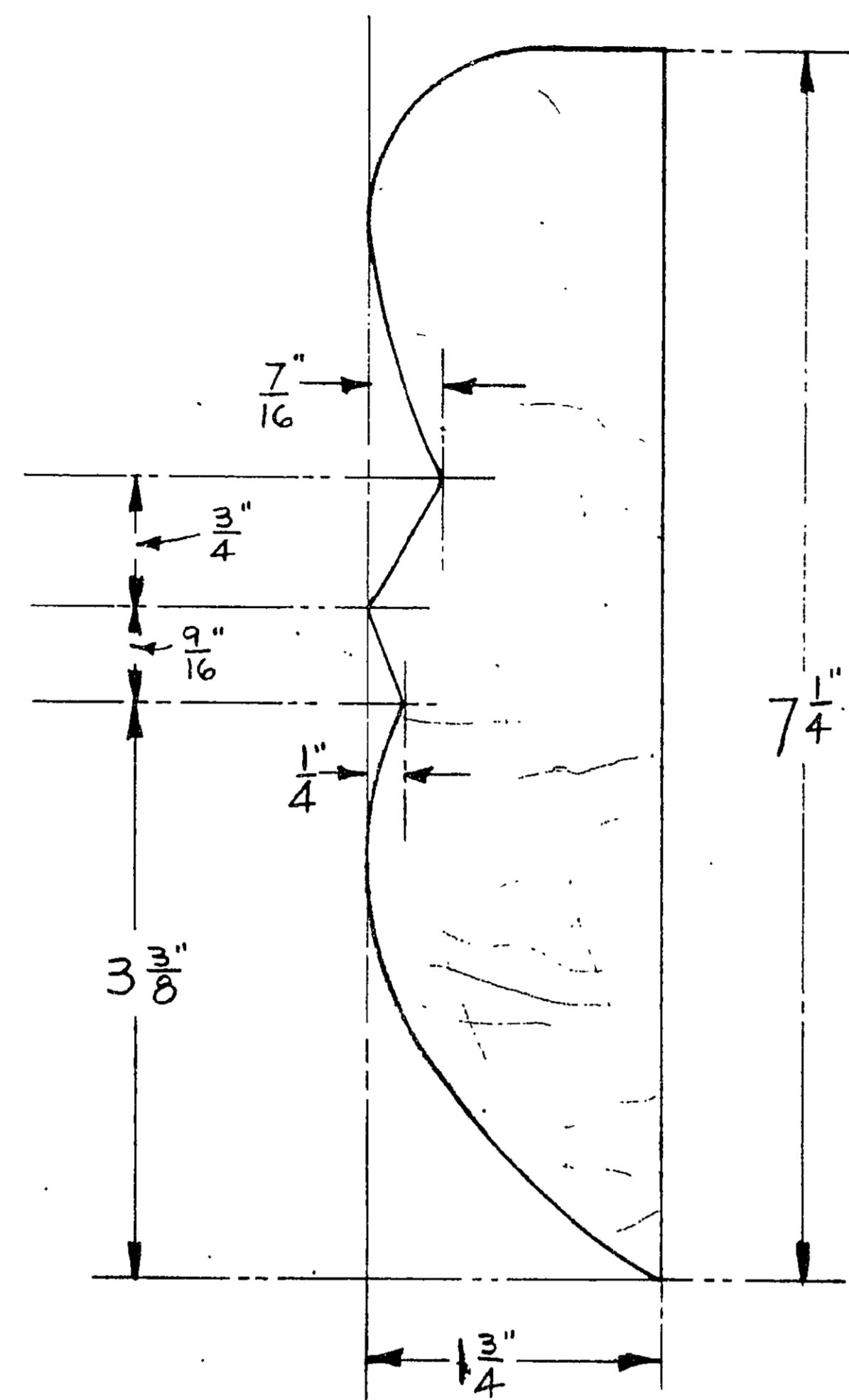
SECTION OF FIRST MOULDING BELOW GUN DECK GUNPORT AT STERN SCALE: FULL SIZE LENGTH 39 FT 0" - ONE REQ'D WHITE OAK
