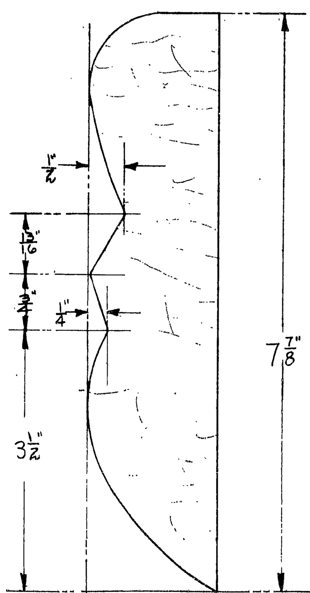
SECTION OF SECOND MOULDING BELOW GUN DECK GUNPORT AT STERN SCALE: FULL SIZE
