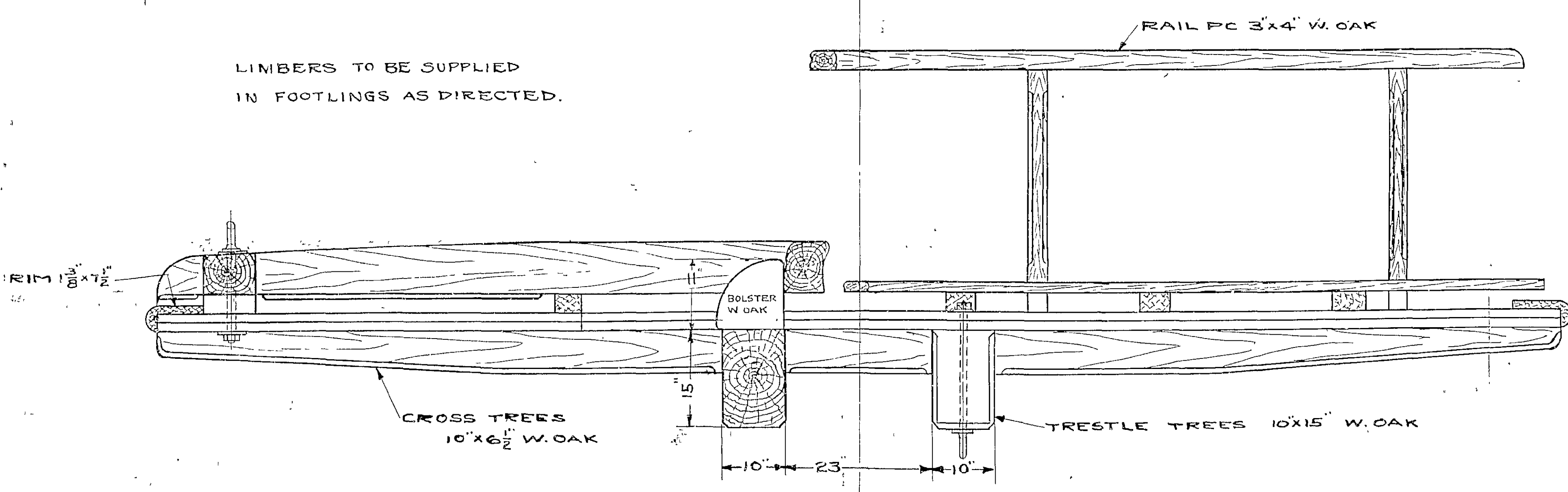
FORE TOP SCALE 3/4" = 1 FT
