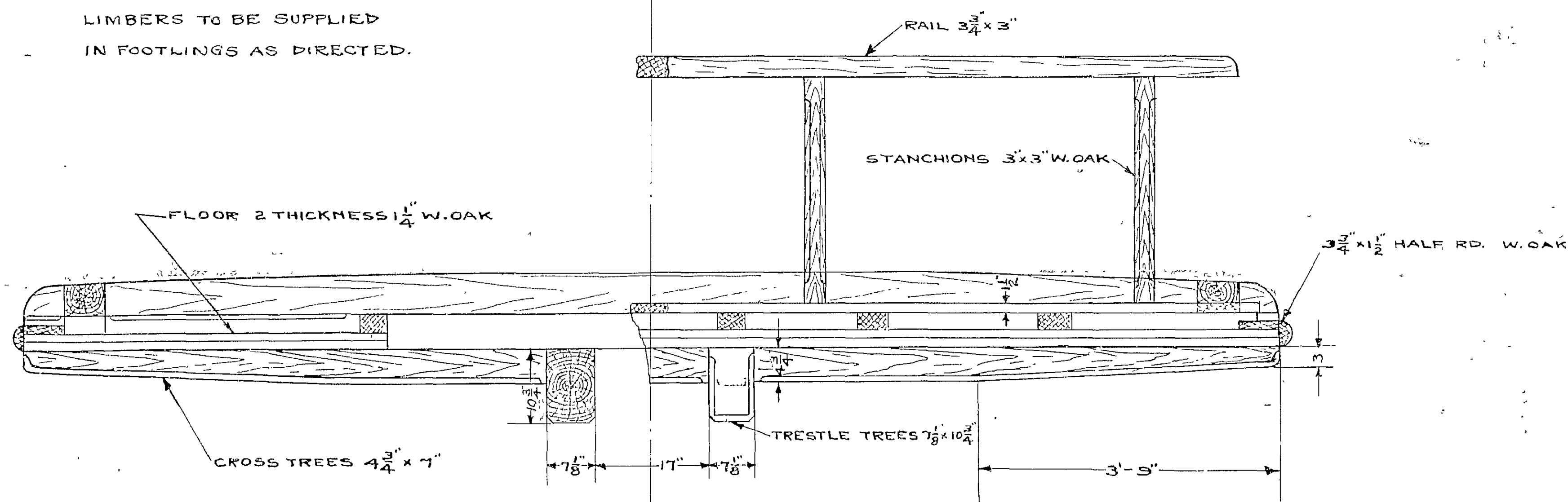
MIZZEN TOP SCALE \frac{3}{4} "=1 FT.
