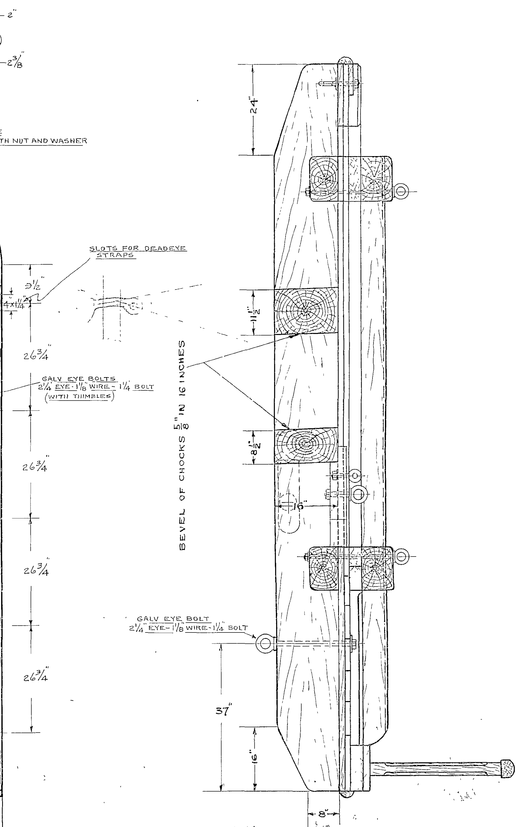
SECTION AA SCALE 3/4" = 1 FT
