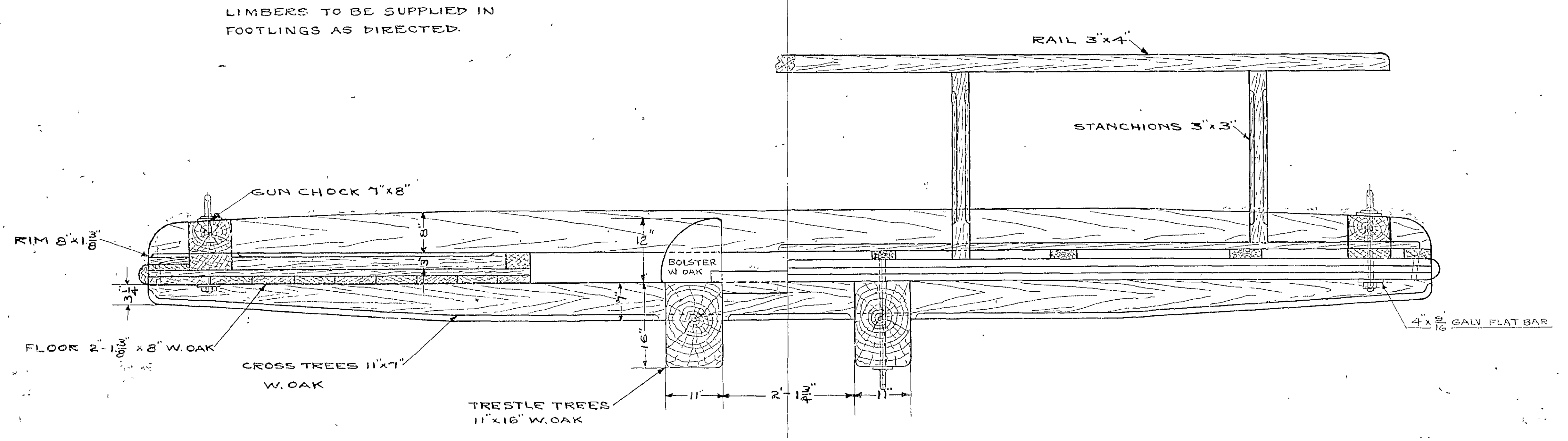
MAIN TOP SCALE 3/4" = 1 FT.
