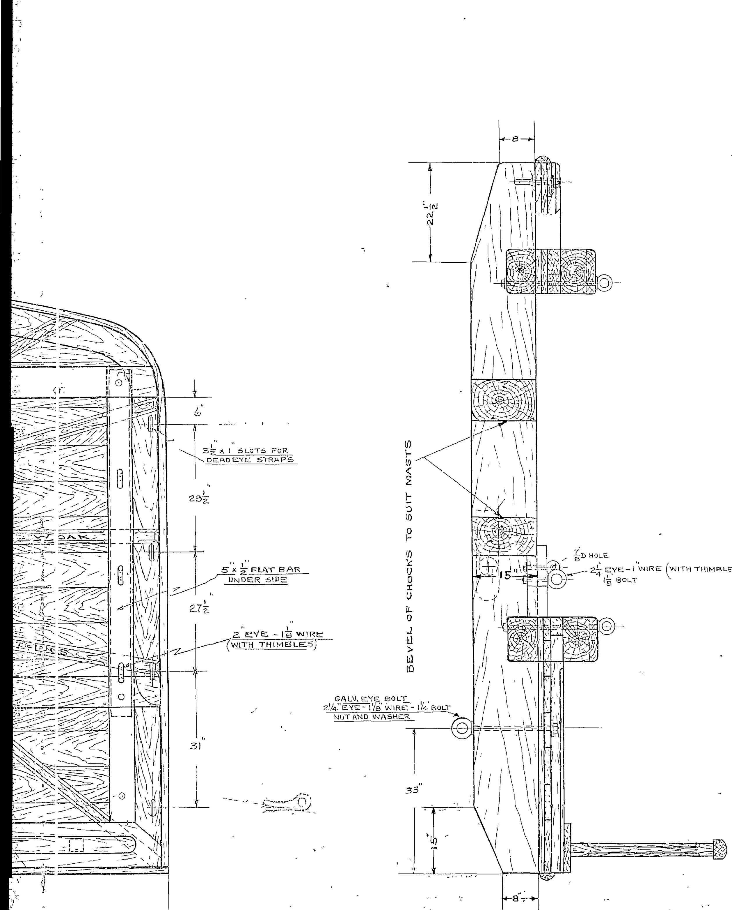
SECTION A-A SCALE 3/4" = 1 FT
