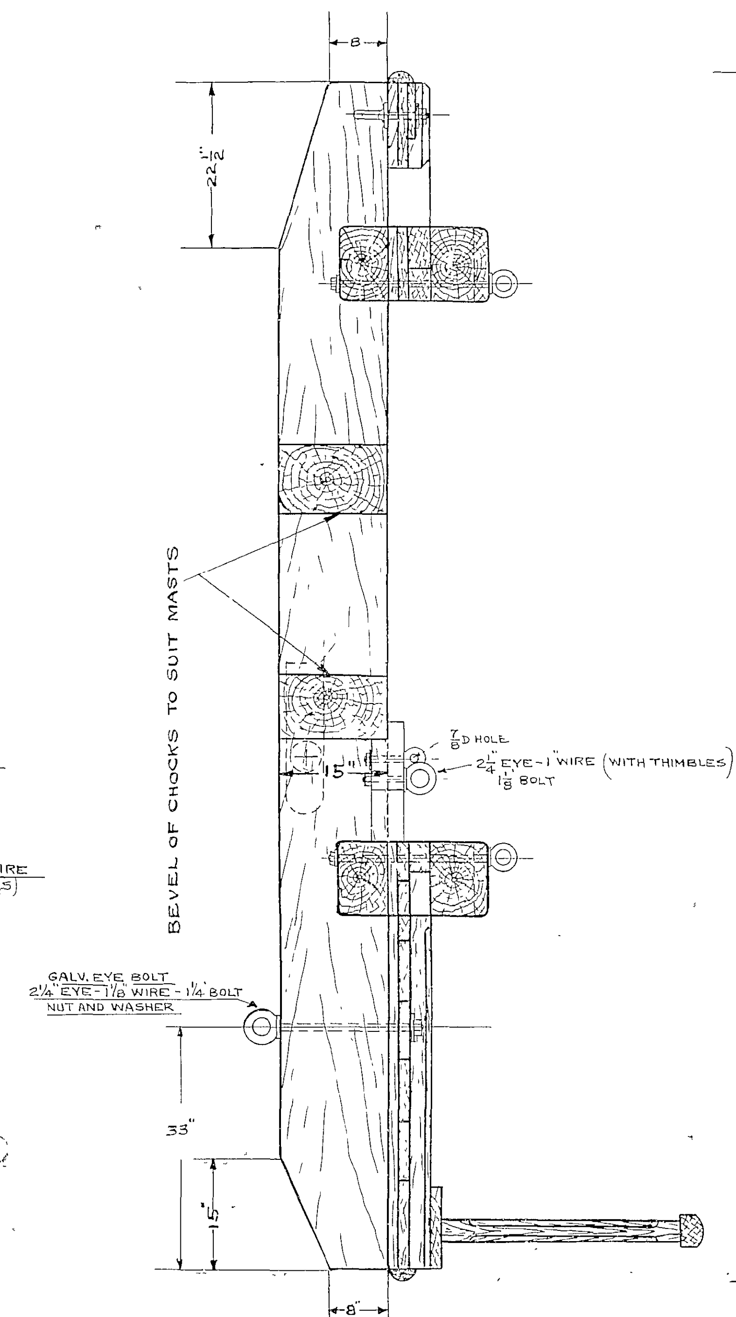
SECTION A-A SCALE \frac{3}{4} "=1 FT.
