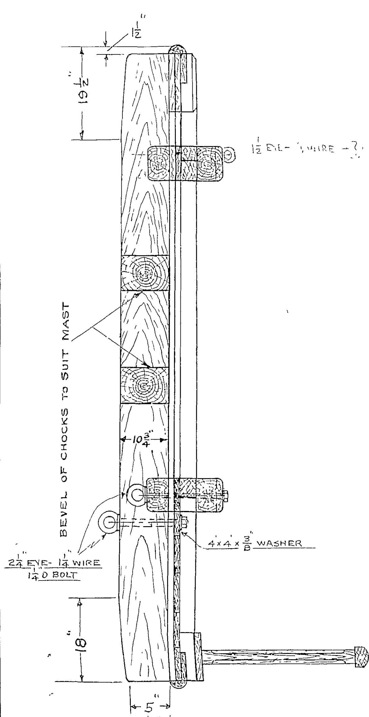
SECTION A-A. SCALE \frac{3}{4} "=1 FT.
