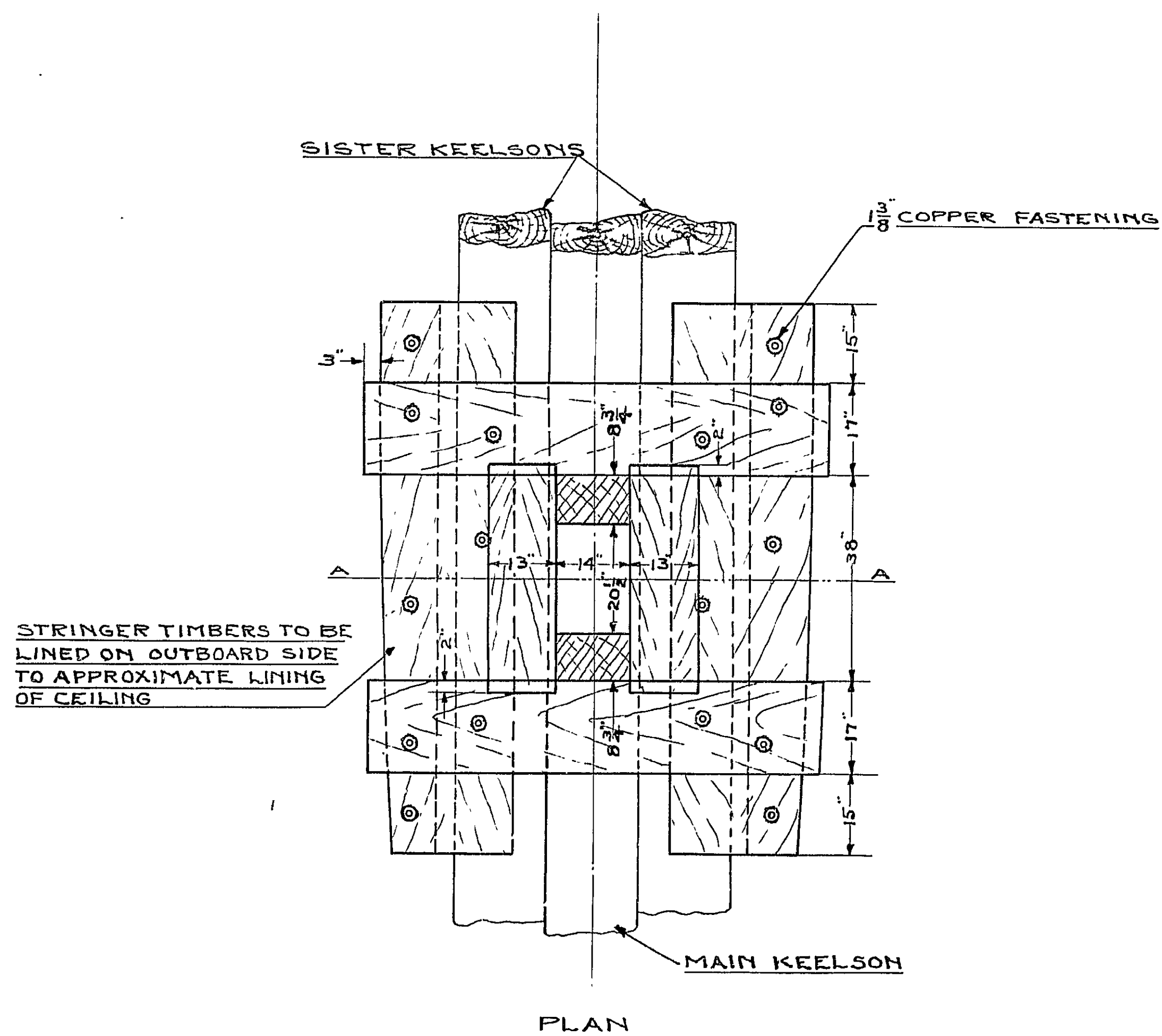
PLAN
