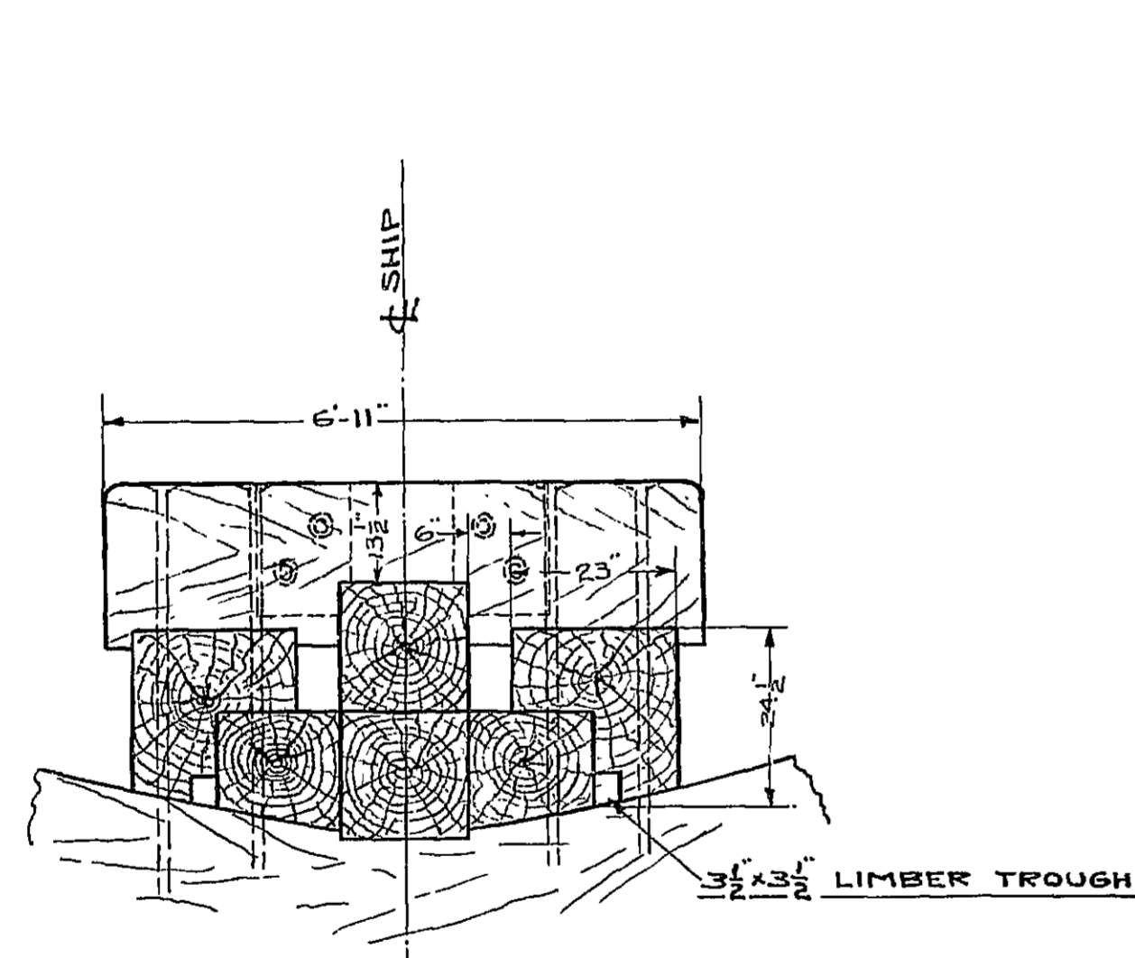
ELEVATION-LOOKING AFT.
