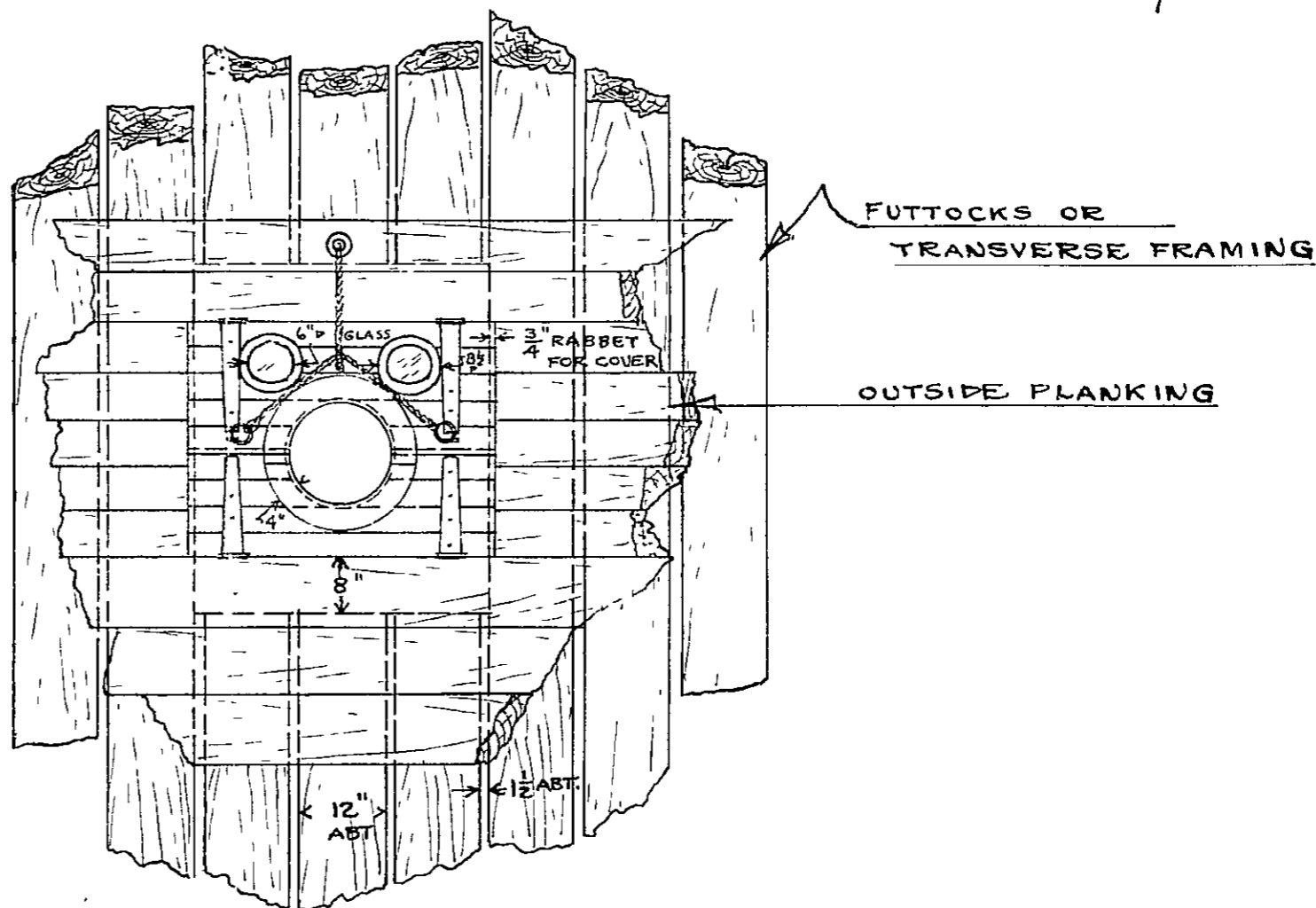
OUTBOARD ELEVATION LOOKING TO PORT OR STBD. MIDSHIP GUN PORT WITH GUNPORT COVERS CLOSED
