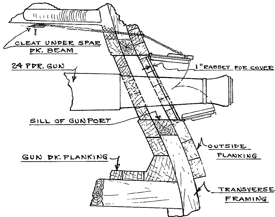
ELEVATION LOOKING FORD. & AFT. SECTION THRU \phi OF GUN PORT. WITH GUNPORT COVERS OPENED
