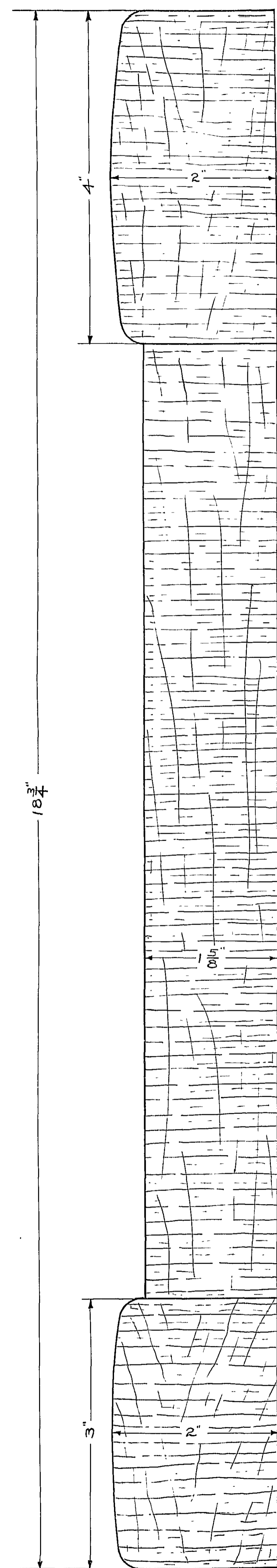
SECTION OF MOLDING & TRAIL BOARD AT THE SHIP SCALE FULL SIZE
