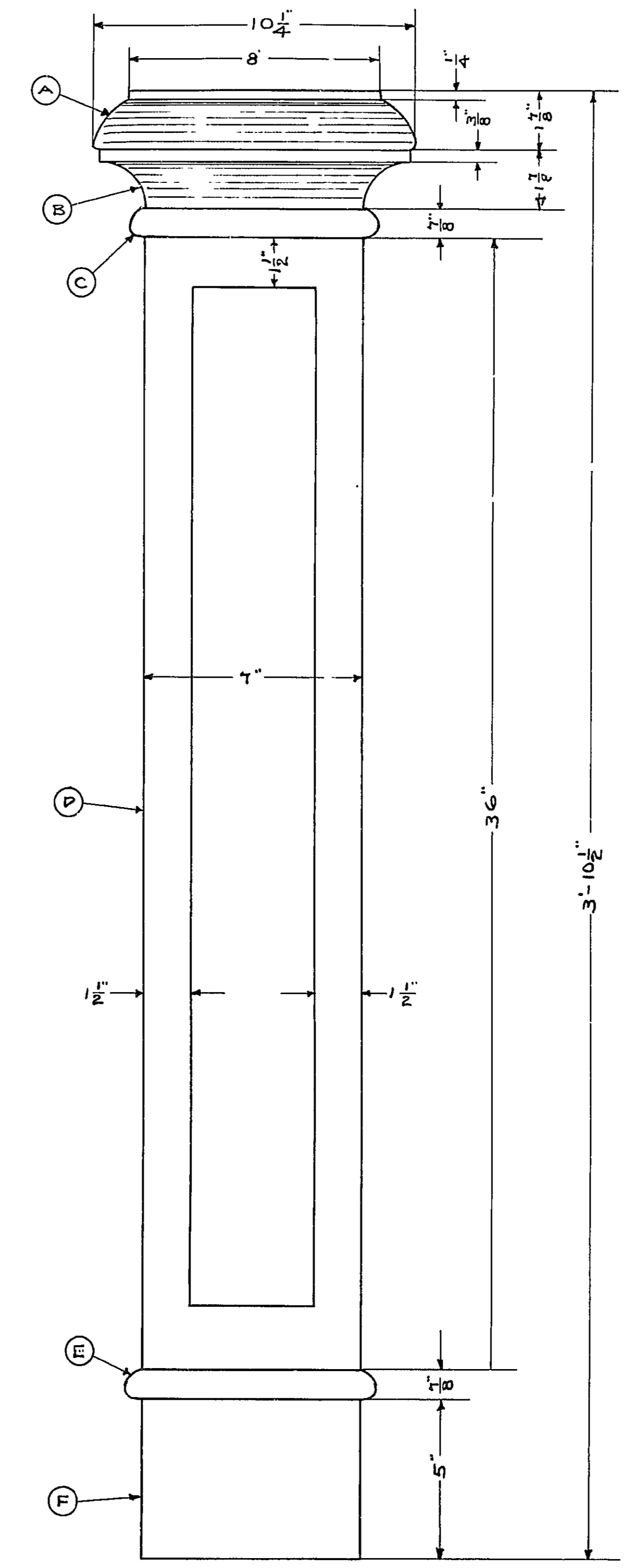
ELEVATION TYPICAL PILASTER SCALE: 3"=1 FT.
