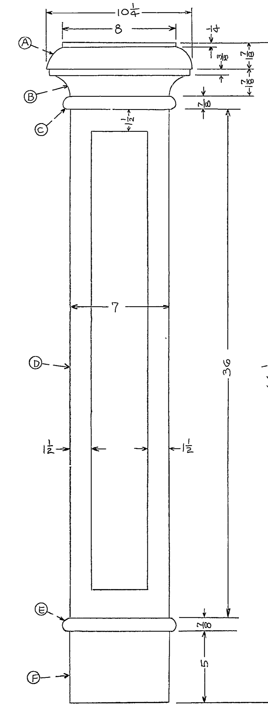
TYPICAL PILASTER ELEVATION SCALE: 3"=1'-0"
