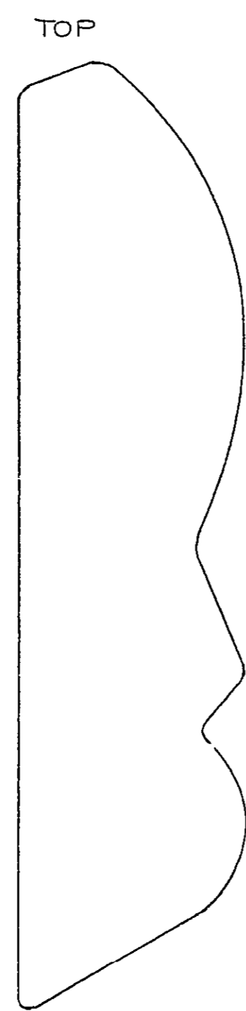
SECTION OF MOLDING BELOW GUN DK STERN PORTS SCALE: FULL SIZE
