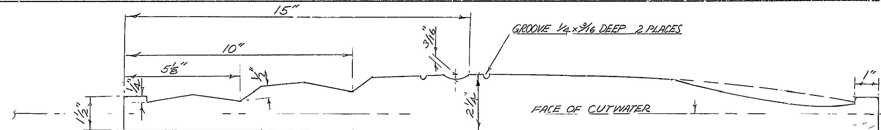
SECT A-A HALF SIZE
