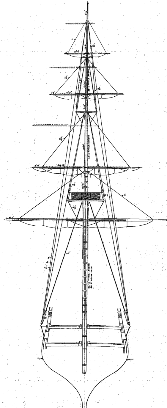
SECTION AT MIZZENMAST LOOKING FORWARD
