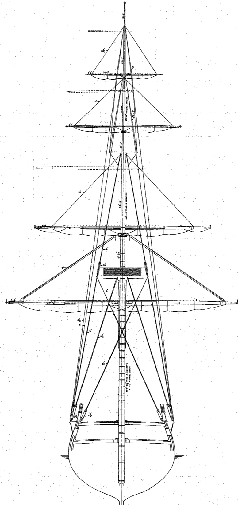
SECTION AT MAINMAST LOOKING FORWARD
