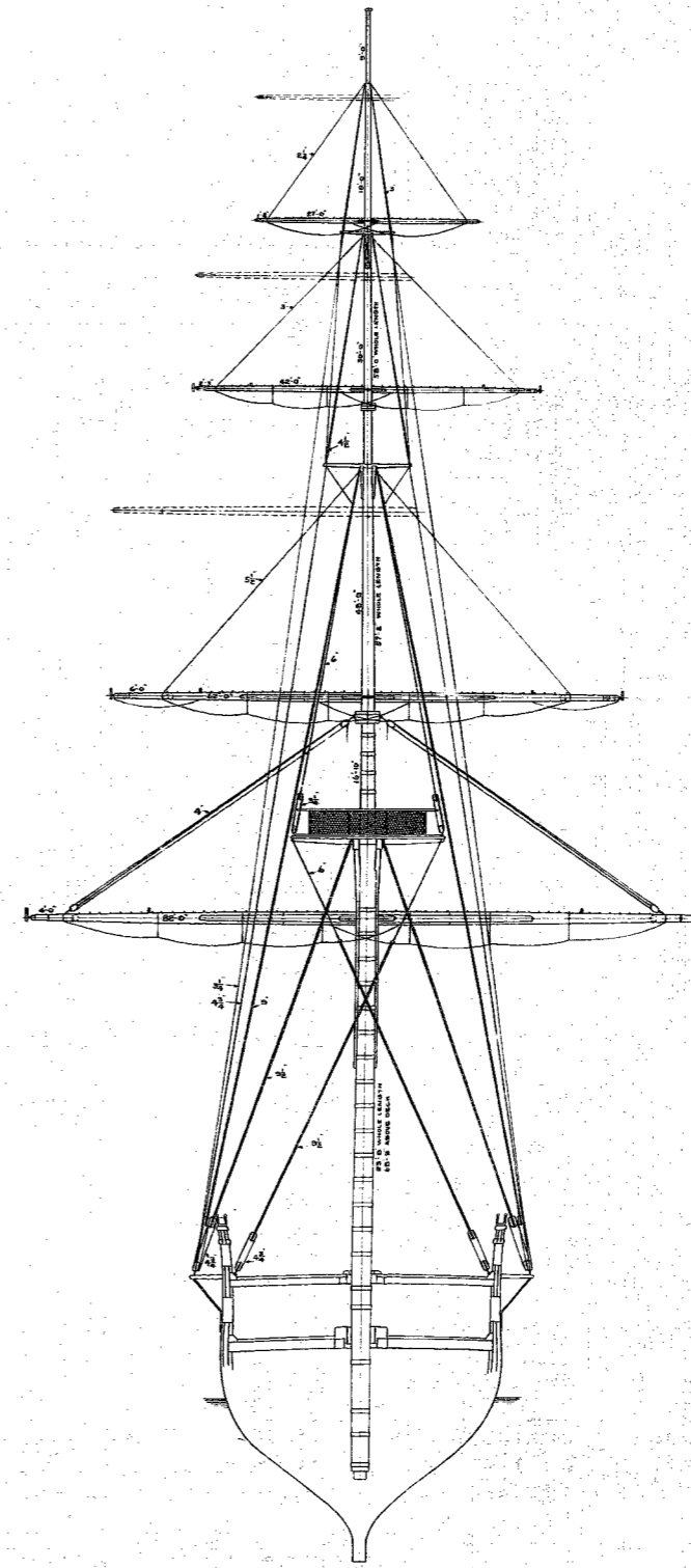
SECTION AT FOREMAST LOOKING FORWARD
