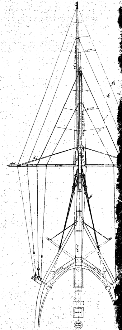
HEAD RIGGING PLAN VIEW
