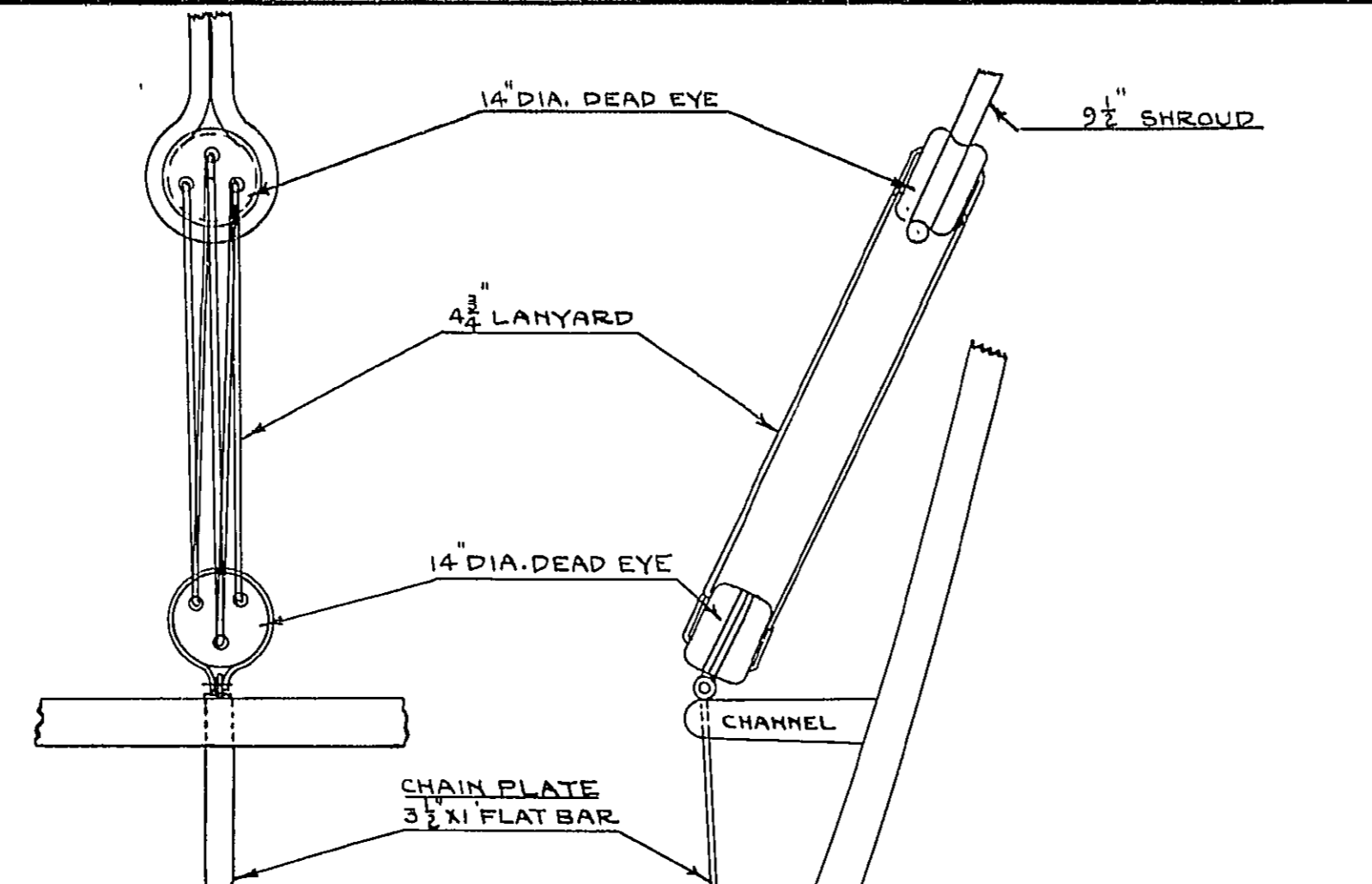
PROFILE VIEW SCALE: 1/2" = 1 FT.
