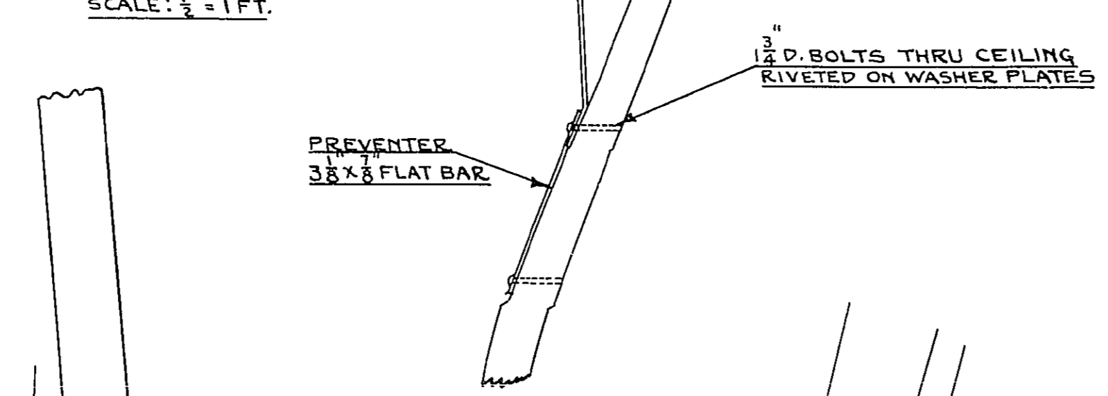
SECTION AT MAINMAST SCALE: 1/2" = 1 FT.
