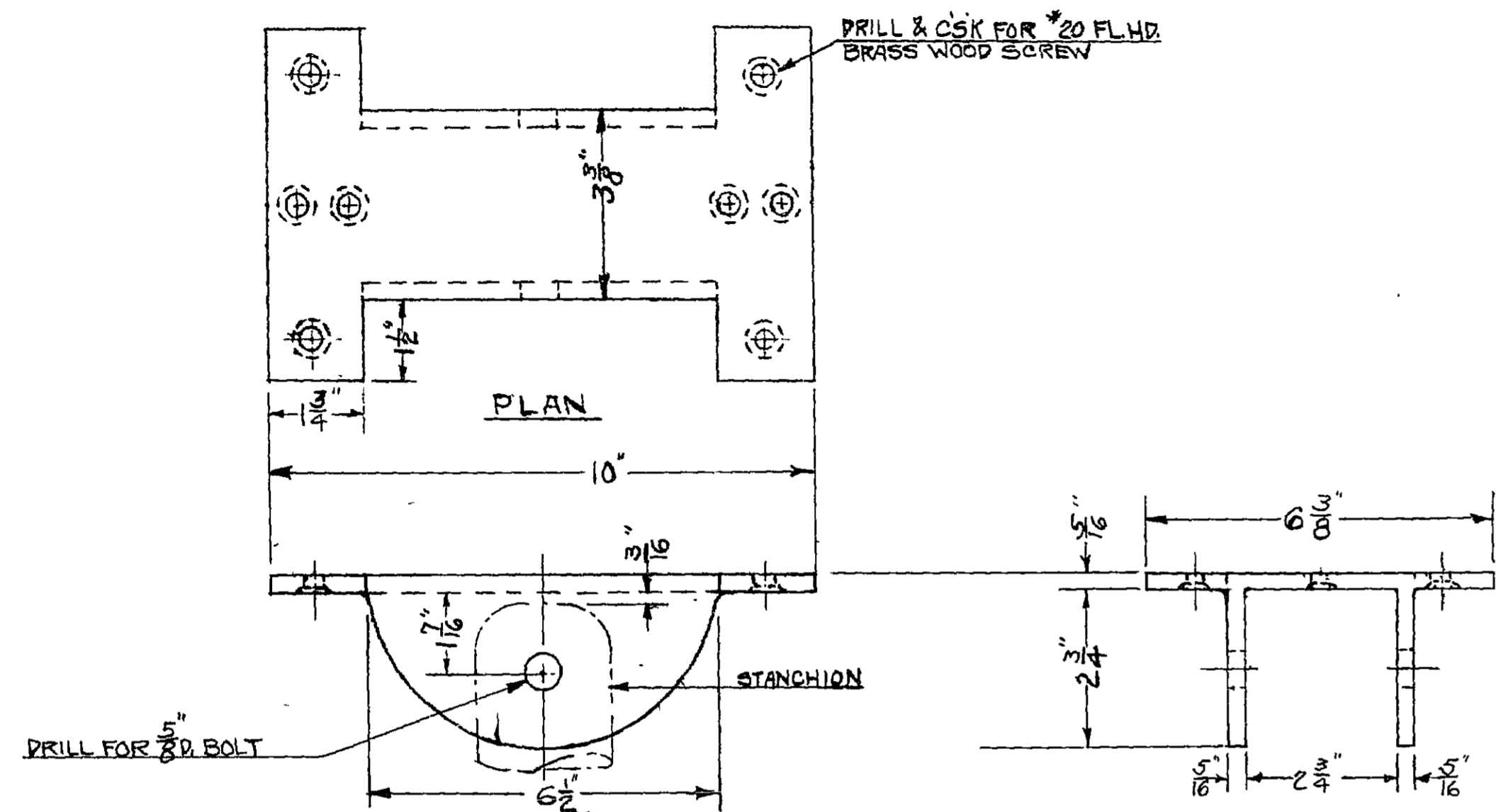
STANCHION HEAD SOCKET MAKE 4 - WROUGHT IRON SCALE 6" = 1 FT.
