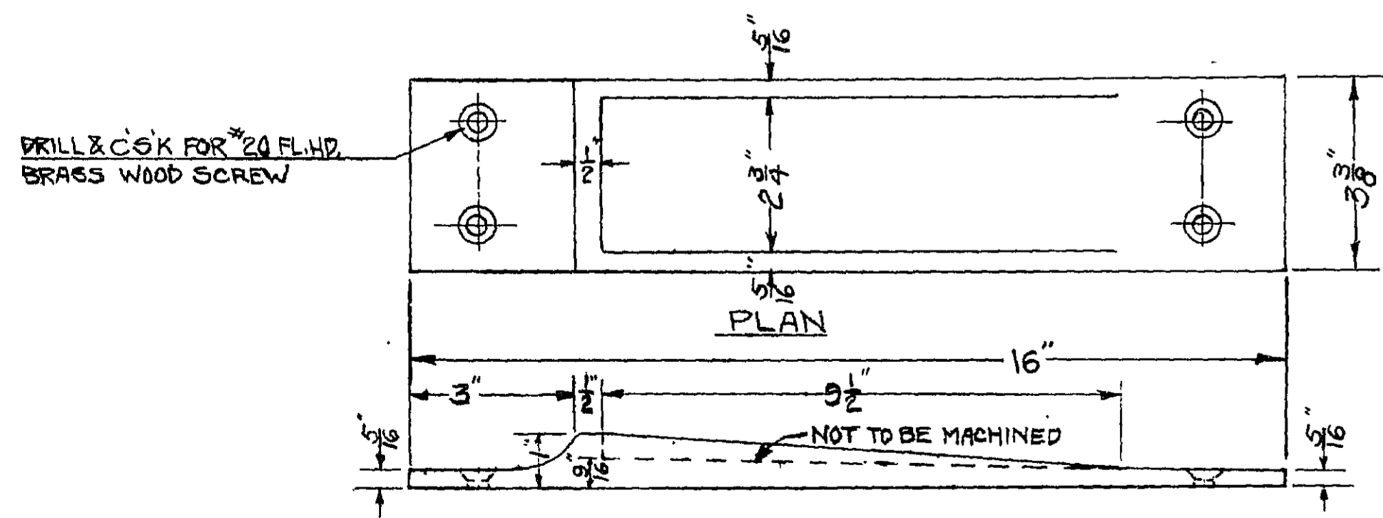
STANCHION FOOT SOCKET MAKE 4 - WROUGHT IRON SCALE 6" = 1 FT.
