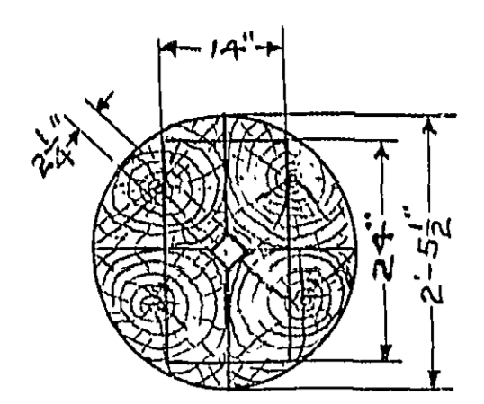
HEEL PLAN SHOWING TENON TO MAST STEP
