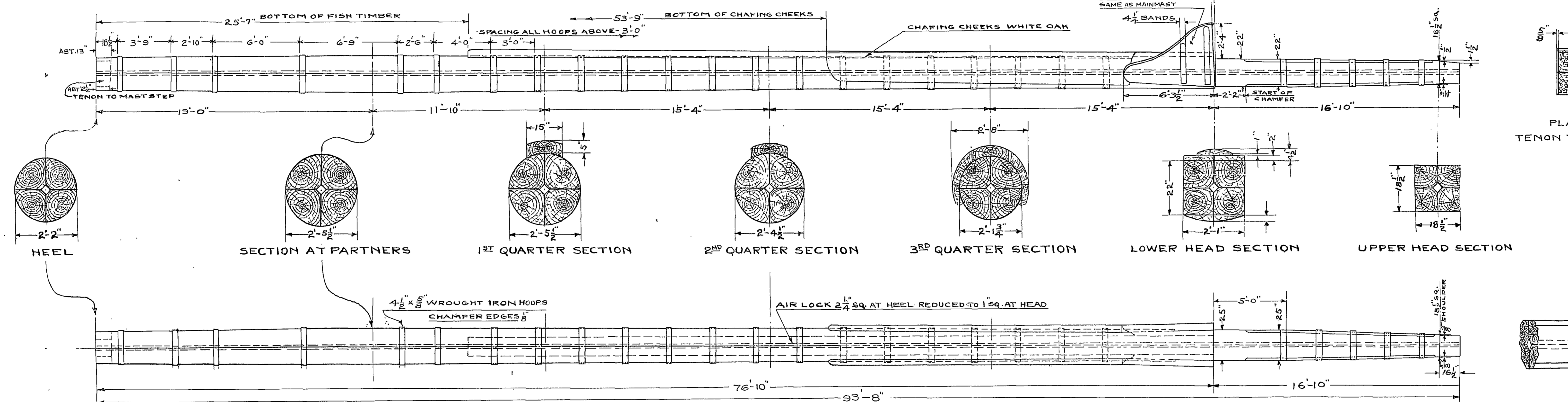
FORE LOWER MAST RAKE 1/16" PER FOOT FROM BOTTOM OF KEEL SCALE: 1/2" & 3/4" = 1 FT.
