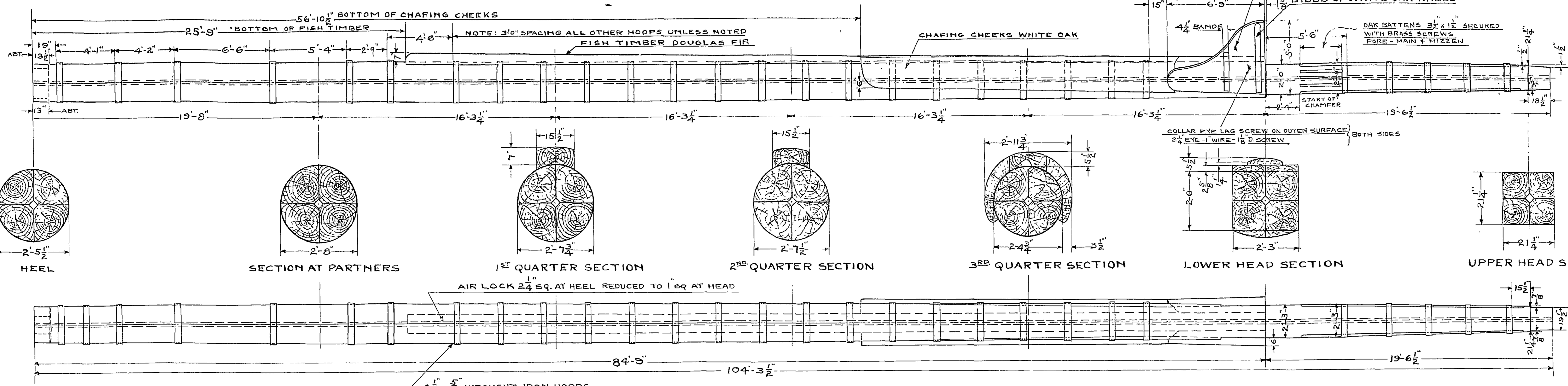
MAIN LOWER MAST RAKE - 3/16" PER FOOT FROM BOTTOM OF KEEL SCALE: 1/2" & 3/4" = 1 FT.
