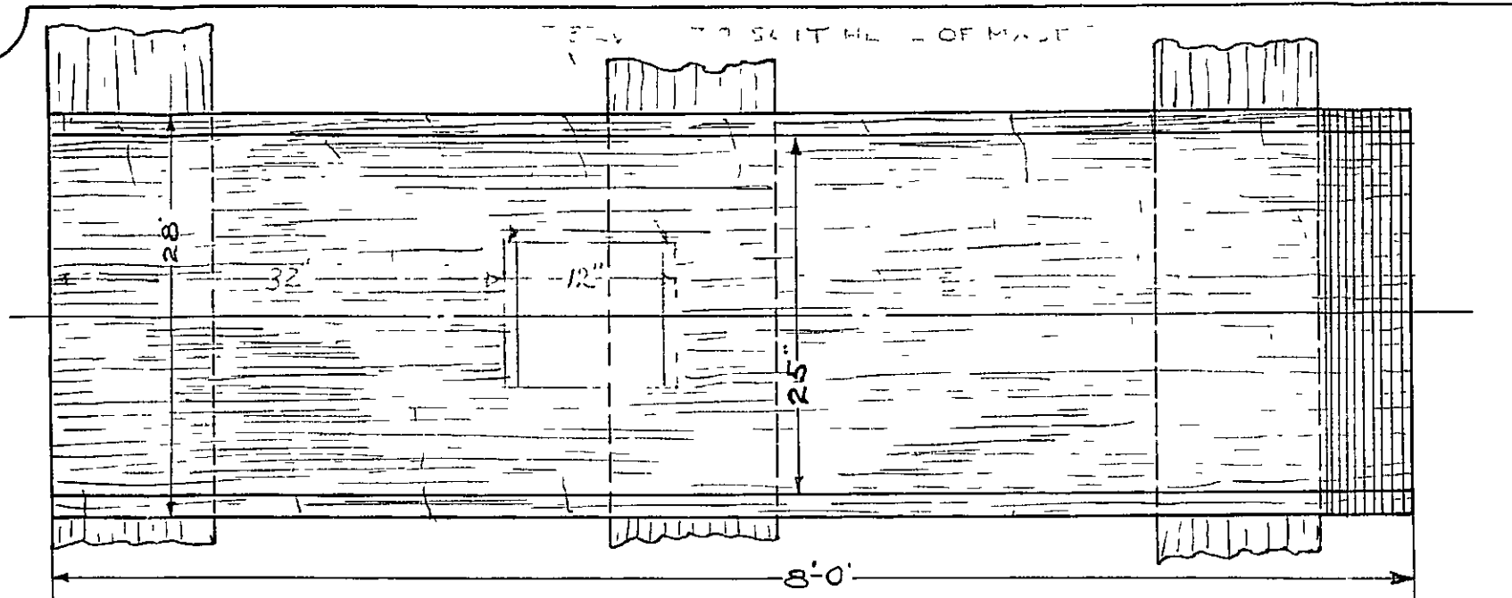
PLAN
